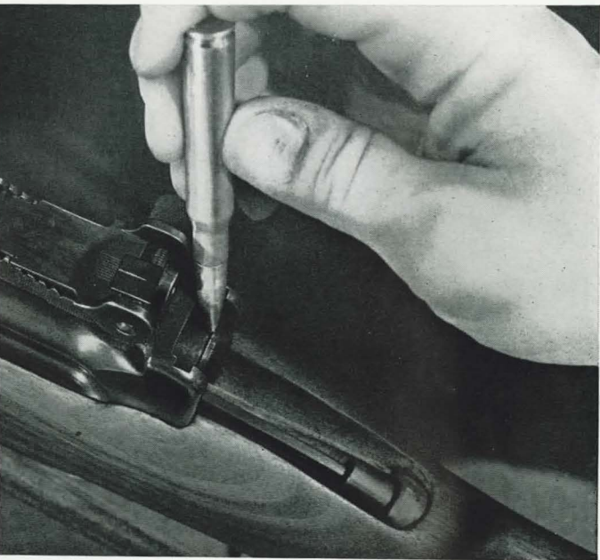
Fig. 7 —Removing the bolt stop with the point of a cartridge.
