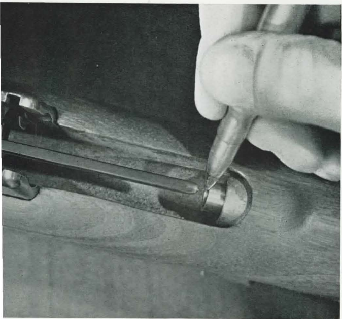
link from the mainspring plunger by compressing the plunger with the point of a cartridge.
